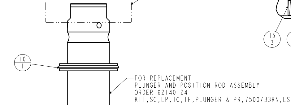
DETAIL A SCALE 1.500
